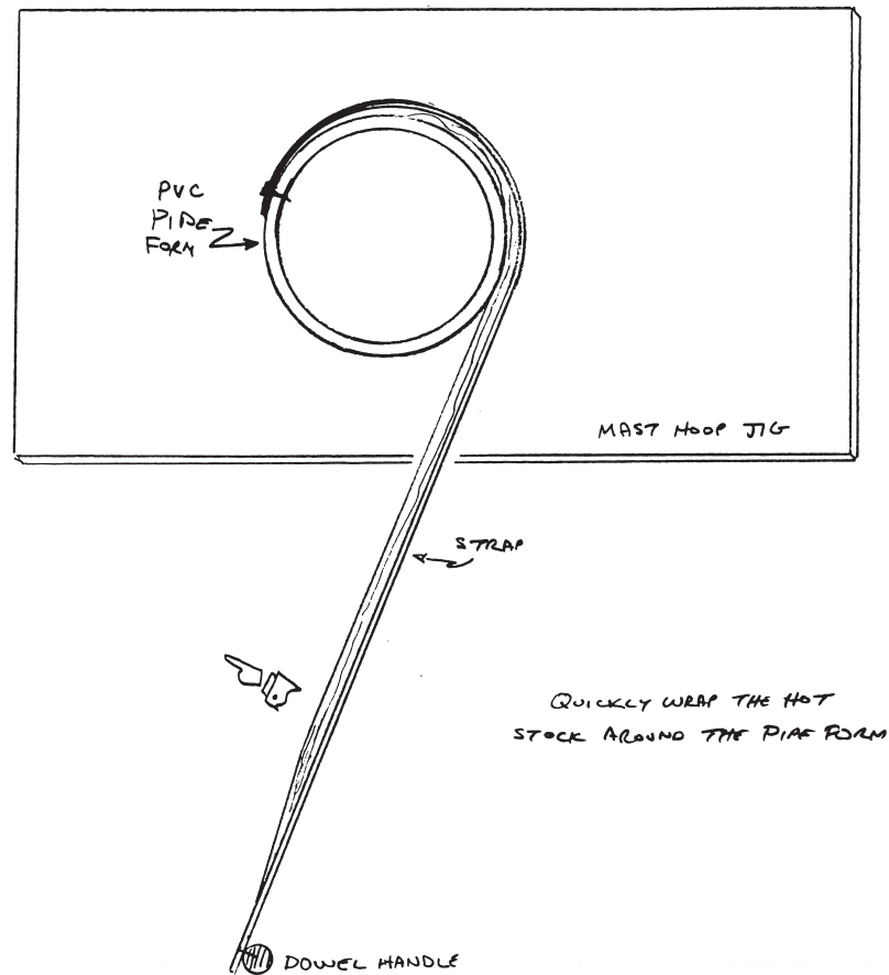
22-10: Bending a mast hoop in a jig step 1.
